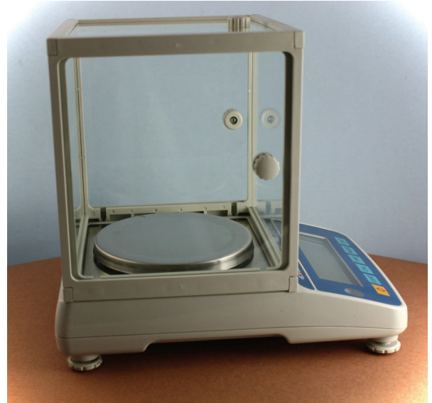
SMT-1008 with included glass draft shield to used to increase accuracy when used in drafty environments
